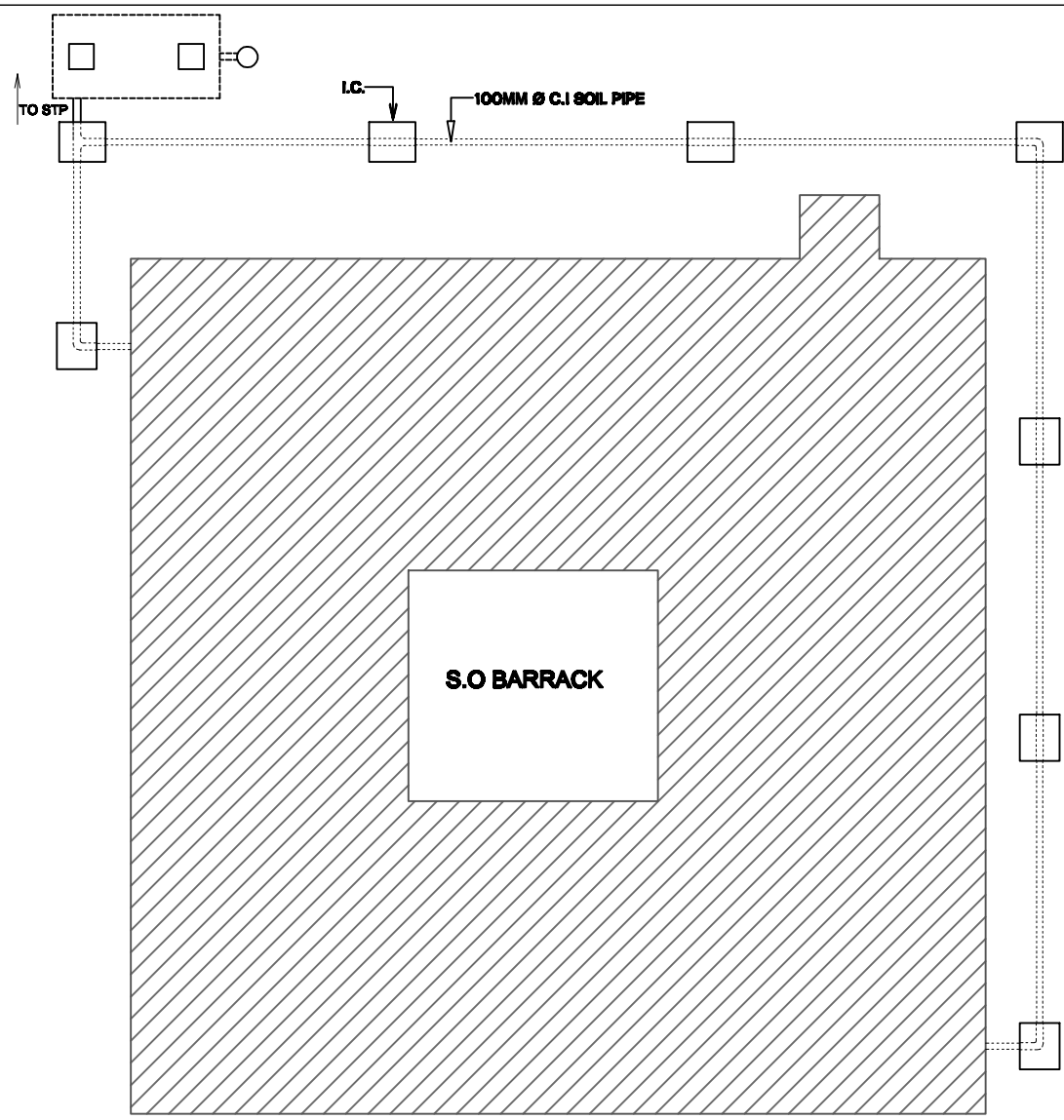
SOIL PIPE LAYOUT PLAN
