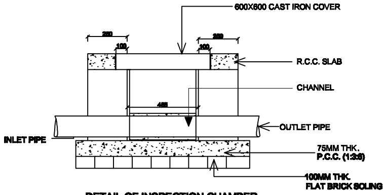
DETAIL OF INSPECTION CHAMBER
