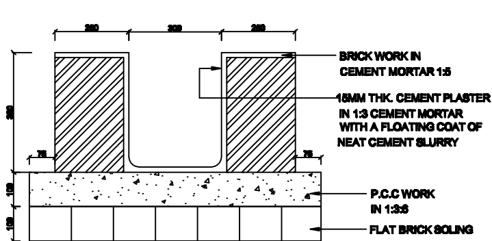
TYPICAL DETAIL OF HOUSE DRAIN
