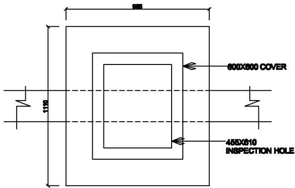
PLAN OF INSPECTION CHAMBER
